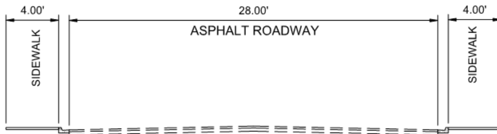
Figure 5: 61 st Street Existing Typical Section
